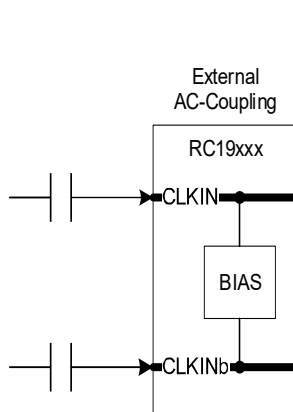
Figure 16. External AC-Coupling
