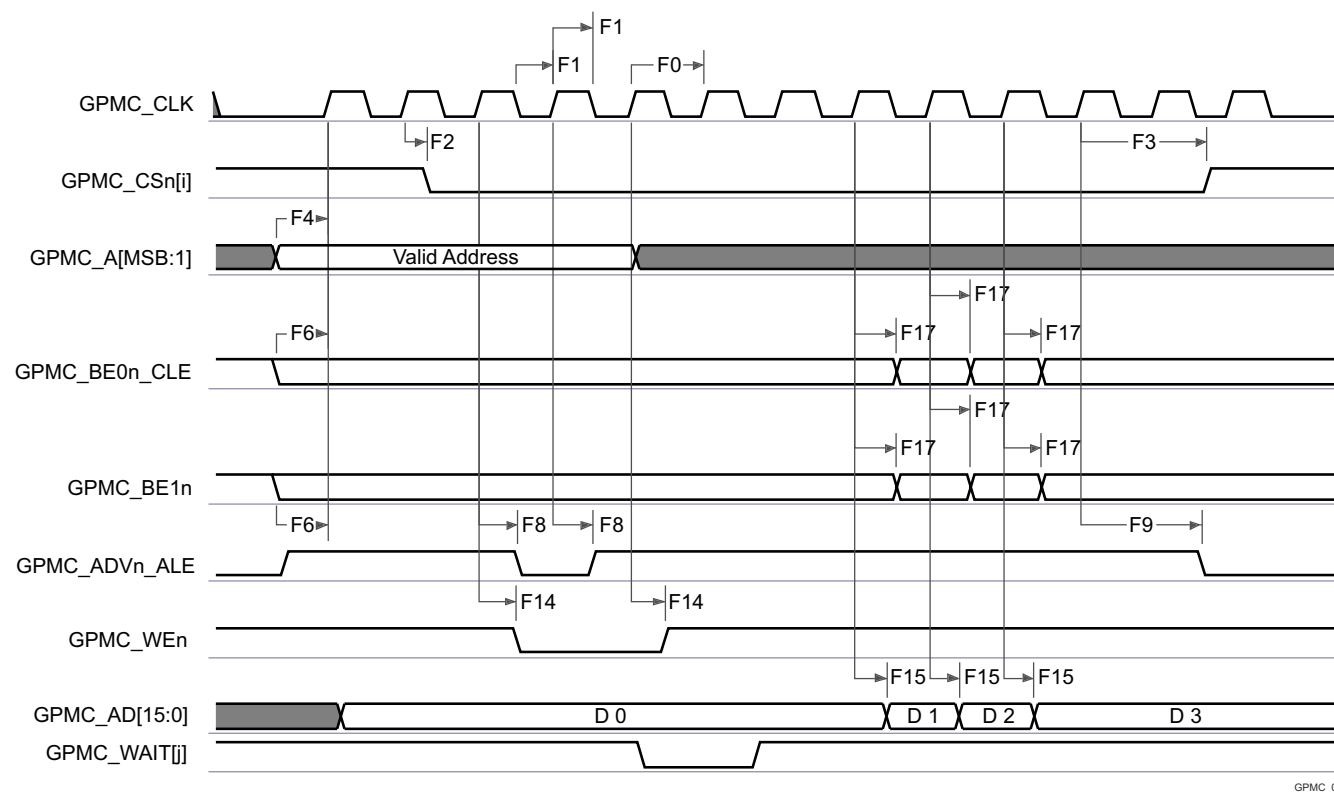
Figure 7-52. GPMC and NOR Flash — Synchronous Burst Read — 4x16-bit (GPMCFCLKDIVIDER = 0)
