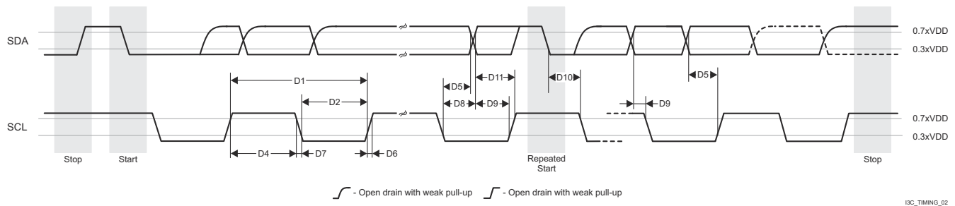
Figure 7-70. I3C Push-Pull Timing (SDR and HDR-DDR Modes)
