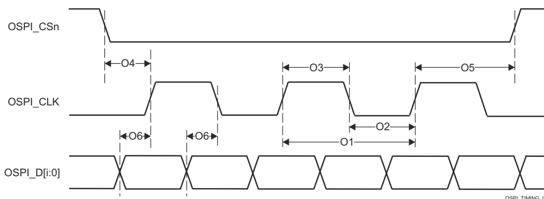
Figure 7-105. OSPI0/1 Switching Characteristics – Tap DDR, No Loopback
