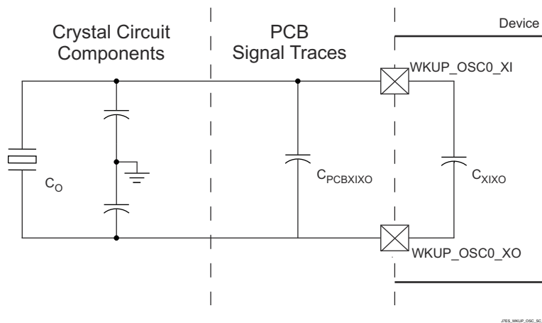
Figure 7-26. Shunt Capacitance
