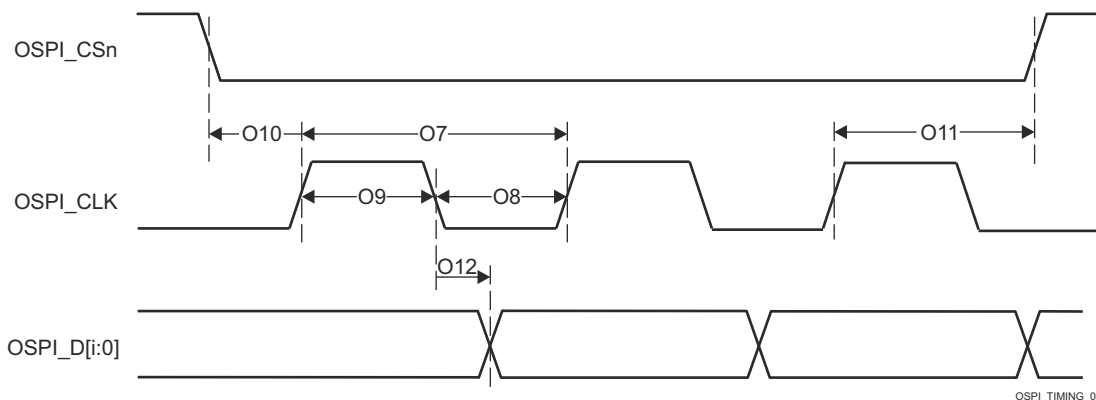
Figure 7-99. OSPI Switching Characteristics – SDR
