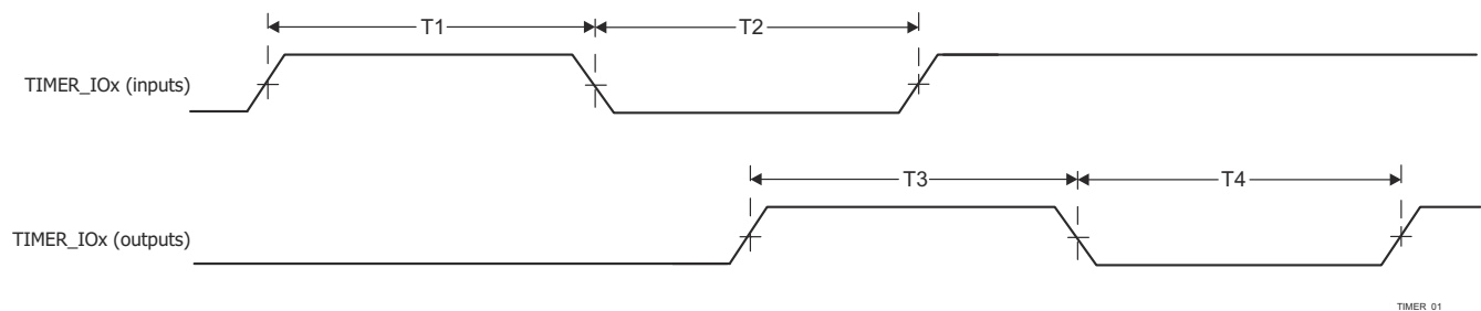
Figure 7-106. Timer Timing
