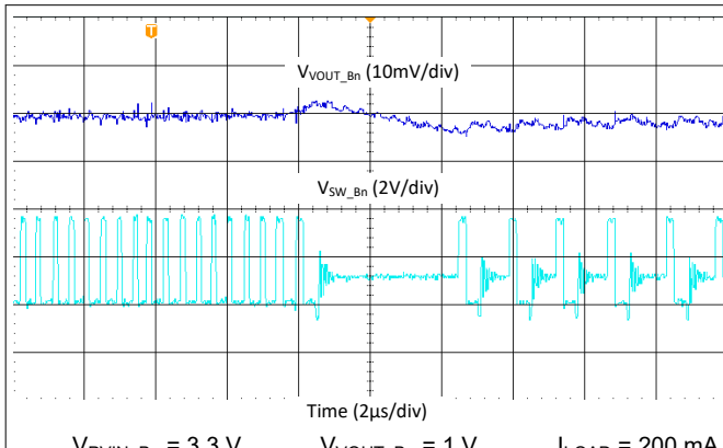
Figure 9-34. Buck Transient from PWM mode to PFM mode, 2.2 MHz, Single Phase
