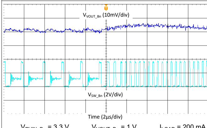
Figure 9-36. Buck Transient from PFM mode to PWM mode, 2.2 MHz, Single Phase
