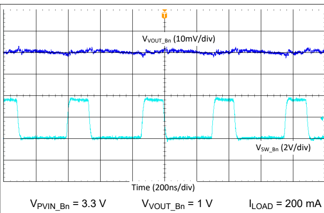
Figure 9-23. Buck Output Ripple - Single Phase, Fsw = 2.2 MHz, Forced-PWM Mode
