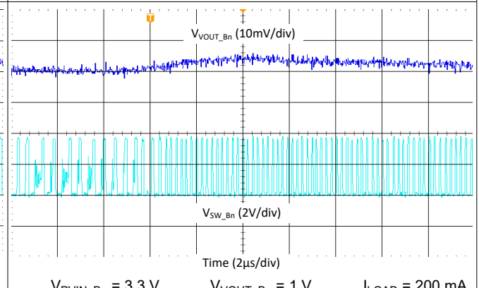
Figure 9-37. Buck Transient from PFM mode to PWM mode, 4.4 MHz, Single Phase
