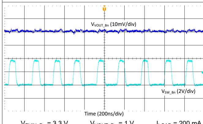
Figure 9-24. Buck Output Ripple - Single Phase, Fsw = 4.4 MHz, Forced-PWM Mode
