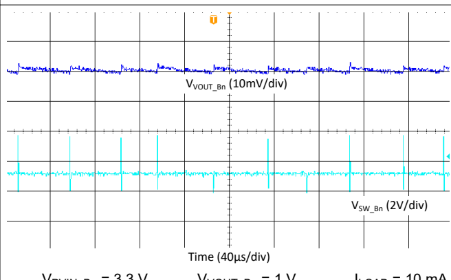
Figure 9-25. Buck Output Ripple - 2-Phase, Auto Mode
