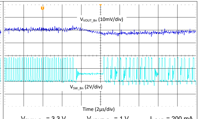
Figure 9-35. Buck Transient from PWM mode to PFM mode, 4.4 MHz, Single Phase
