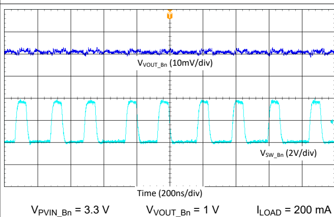
Figure 9-27. Buck Output Ripple - 2-Phase, Fsw = 4.4 MHz, Forced-PWM Mode
