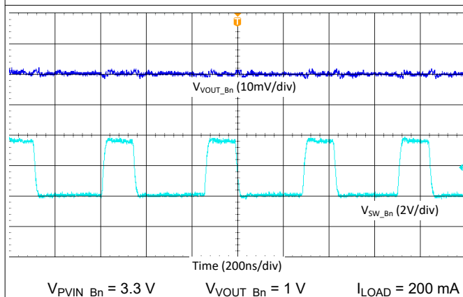
Figure 9-26. Buck Output Ripple - 2-Phase, Fsw = 2.2 MHz, Forced-PWM Mode
