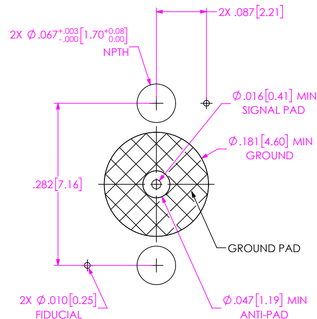
RECOMMENDED PCB LAYOUT (SEE NOTE 2)
