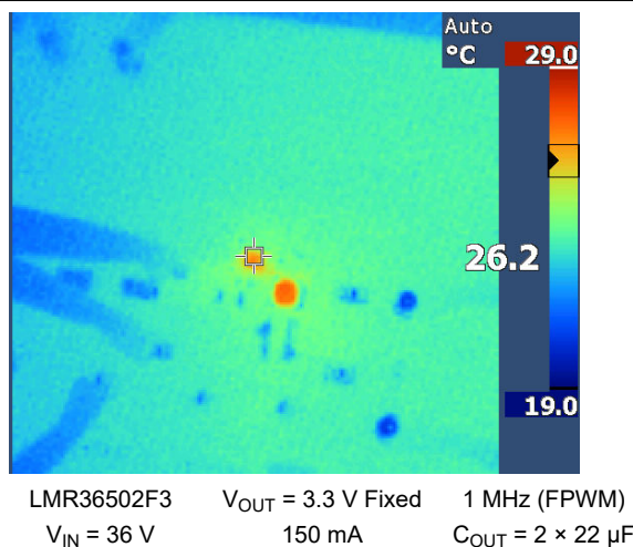
Figure 9-13. Thermal Image
