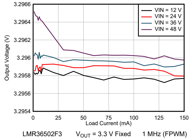
Figure 9-4. Line and Load Regulation
