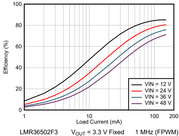
Figure 9-3. Efficiency
