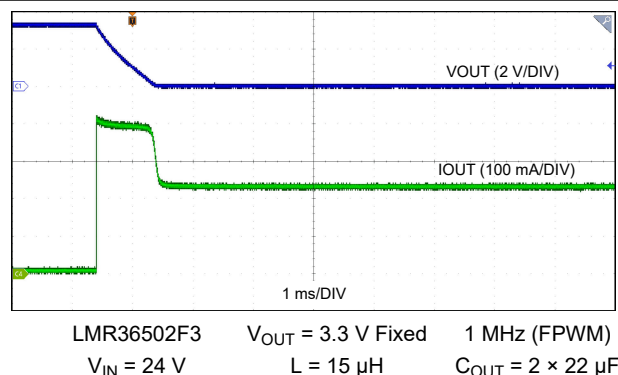
Figure 9-11. Short Circuit Entry
