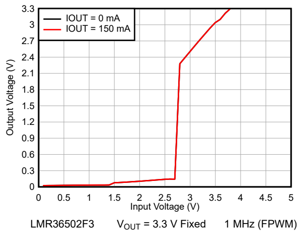
Figure 9-5. Dropout VIN High to Low
