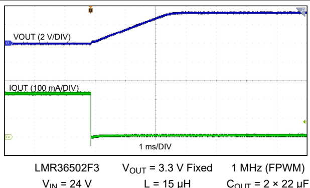
Figure 9-12. Short Circuit Exit
