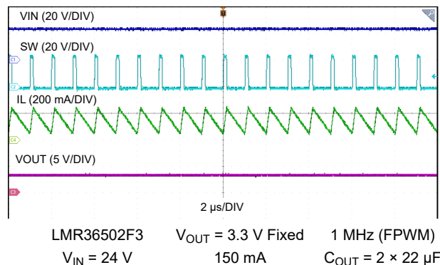
Figure 9-9. Steady State Waveforms
