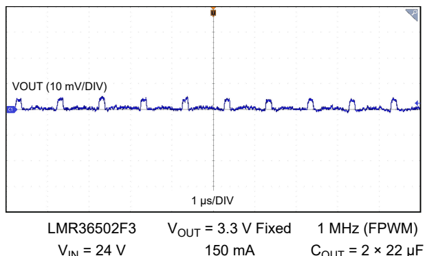
Figure 9-10. Output Voltage Ripple
