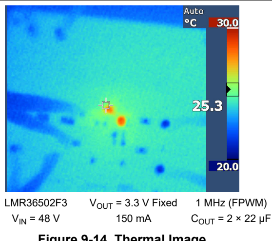
Figure 9-14. Thermal Image
