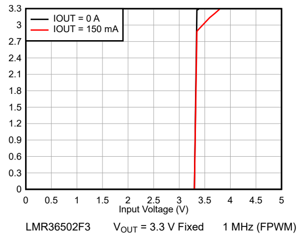
Figure 9-6. Dropout VIN Low to High
