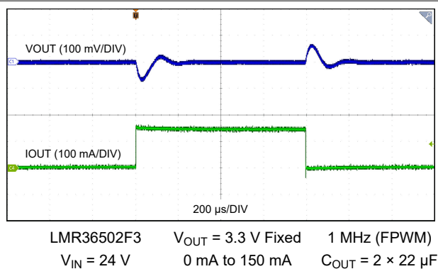
Figure 9-7. Load Transient
