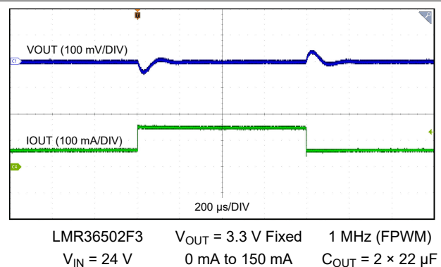
Figure 9-8. Load Transient
