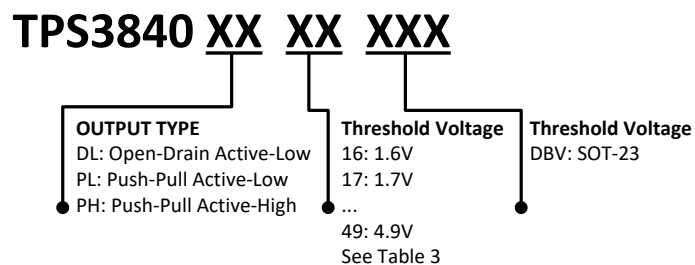
Figure 1. Device Nomenclature
