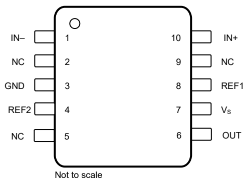
Figure 6-3. INA241x-Q1: DGS Package 10-Pin VSSOP Top View
