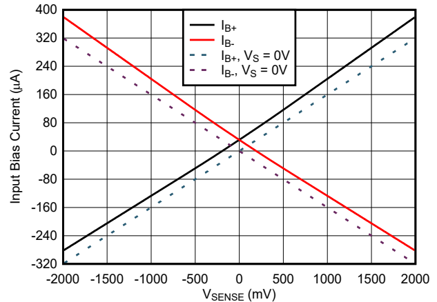
Figure 7-18. INA241x1-Q1 Input Bias Current vs V_{\text{SENSE}}
