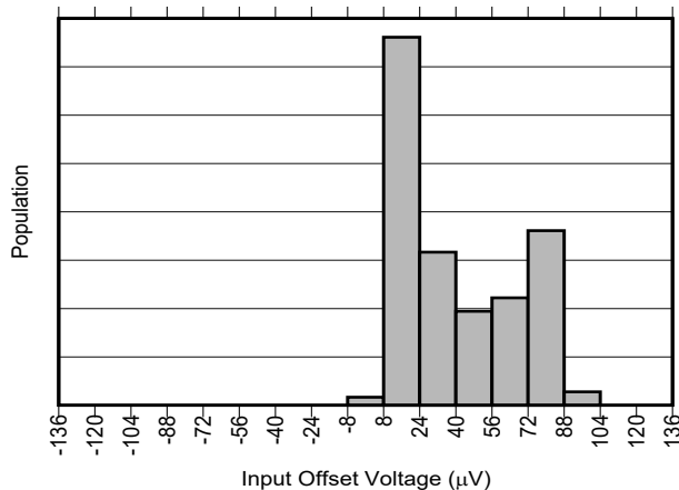
Figure 7-3. INA241A3-Q1 and INA241A4-Q1 Input Offset Production Distribution
