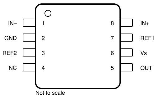
1. D (SOIC) package is preview only. Figure 6-2. INA241x-Q1: D and DGK Package 8-Pin SOIC and 8-Pin VSSOP Top View
