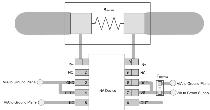
Figure 9-4. INA241x-Q1 10-Pin VSSOP (DGS) Package Recommended Layout
