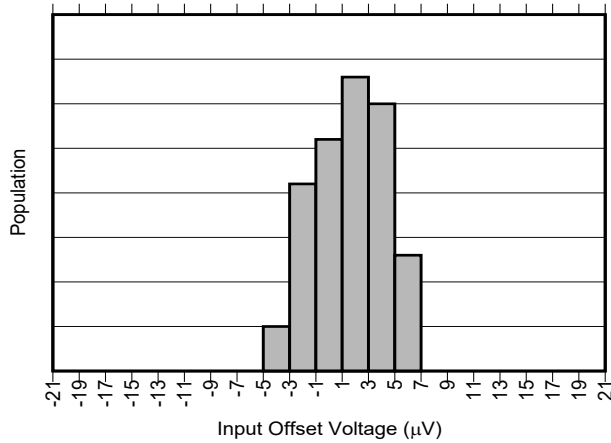
Figure 7-1. INA241A1-Q1 Input Offset Production Distribution
