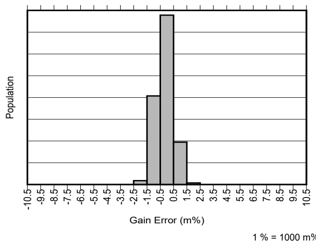
Figure 7-10. INA241A1-Q1, INA241A2-Q1 and INA241A3-Q1 Gain Error Production Distribution
