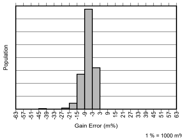
Figure 7-12. All Gains INA241B-Q1 Gain Error Production Distribution
