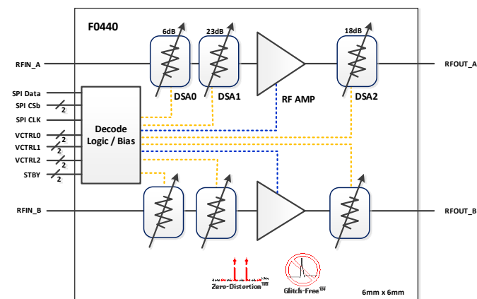
Figure 1. Block Diagram
