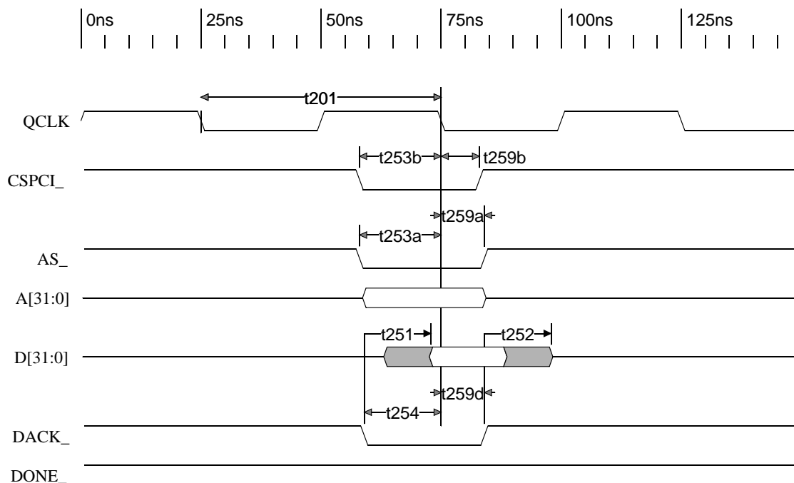
Figure 40: MC68360 IDMA Read — Dual Address, Fast Termination
