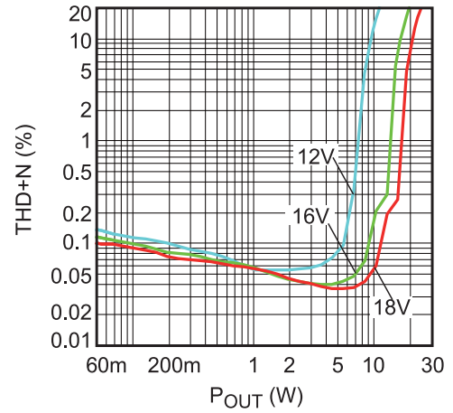
THD+N vs. P_{OUT} (1kHz, 8 \Omega +66 \mu H)
