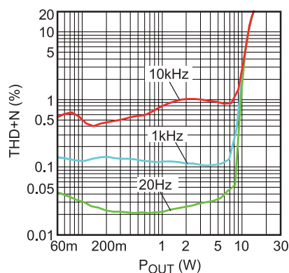
THD+N vs. POUT (12V, 6Ω+44μH)
