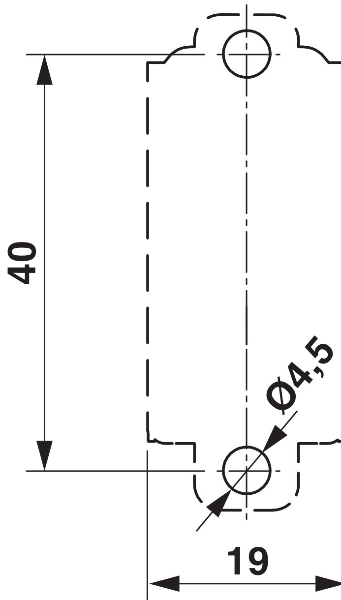
Drilling plan/solder pad geometry
