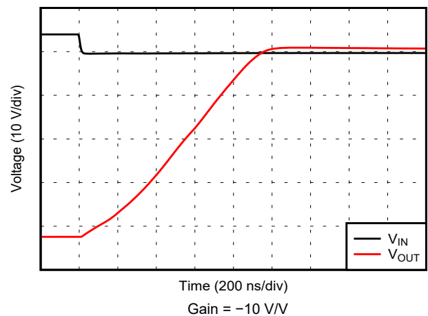
Figure 6-64. Negative Overload Recovery
