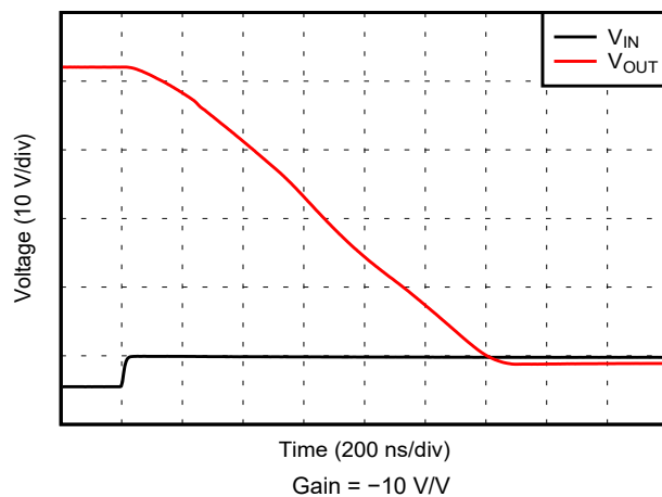
Figure 6-63. Positive Overload Recovery
