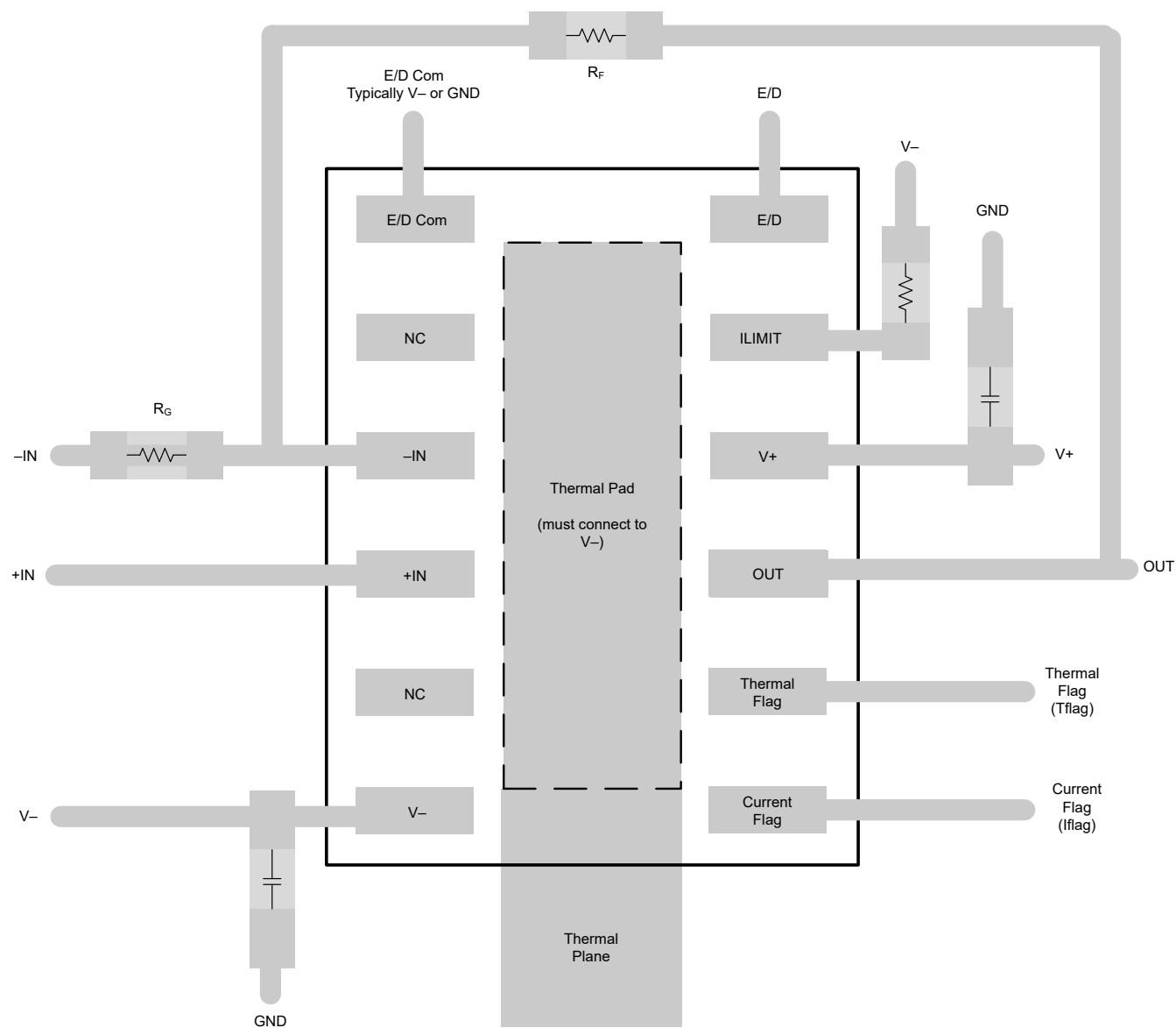
Figure 8-5. OPA593 Board Layout for Noninverting Configuration
