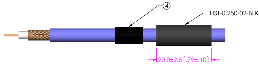
IN-PROCESS 2 ADD HEAT SHRINK TUBE AND FERRULE
