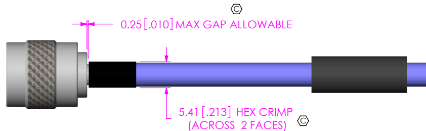
DETAIL 'A' SCALE 2.5:1
