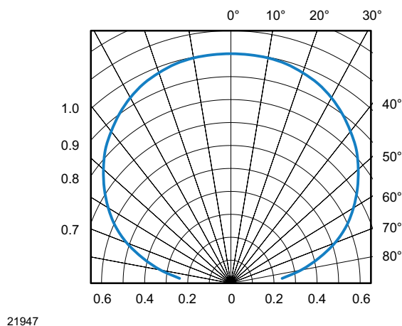
Fig. 9 - Horizontal Directivity
