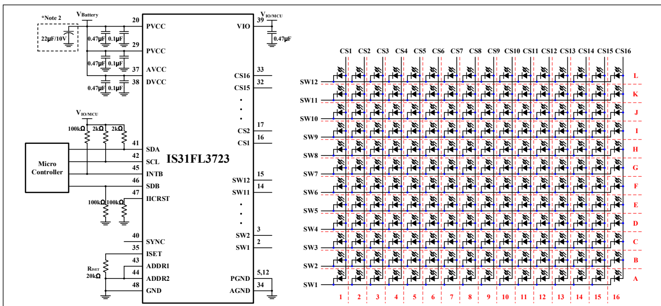
Figure 1 Typical Application Circuit (12×16)
