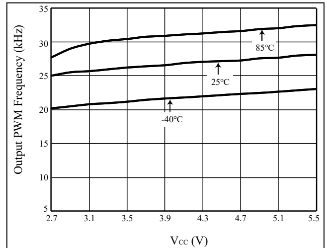
Figure 18 V CC vs. CSx PWM Frequency
