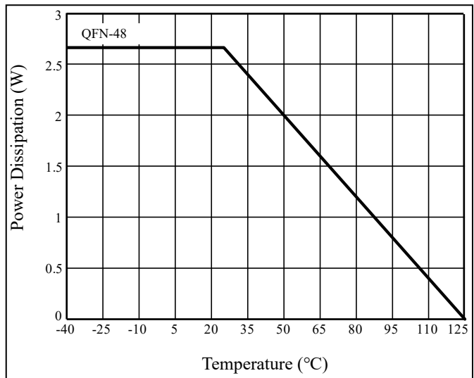
Figure 17 Dissipation Curve
