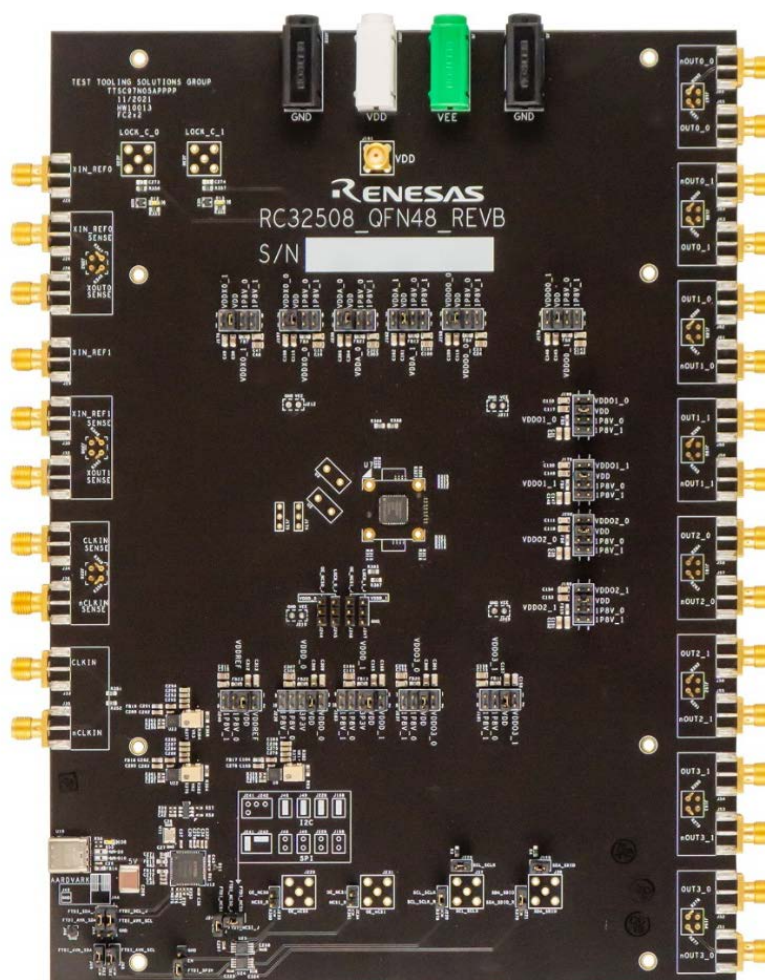
Figure 1. RC32508A Board
