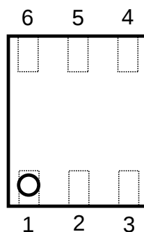
DFN1814-6C Pin Configuration
