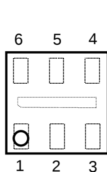
DFN(PLP)1414-6 Pin Configuration
