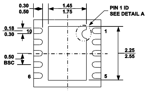
QFN10 (3x3mm)
