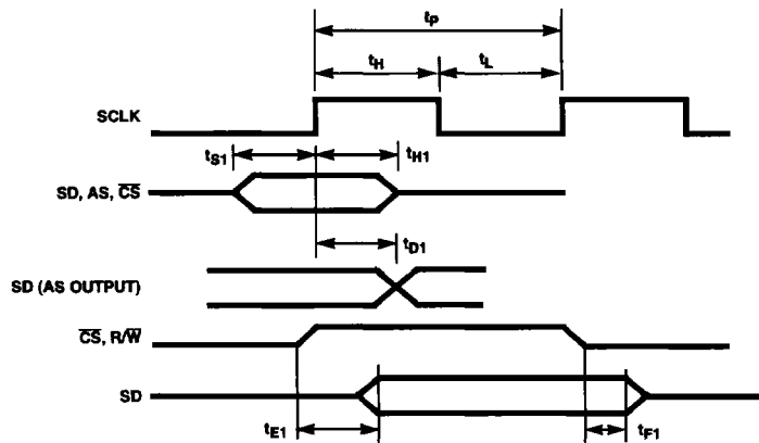
FIGURE 22. SERIAL CONTROL PORT SIGNAL TIMING
