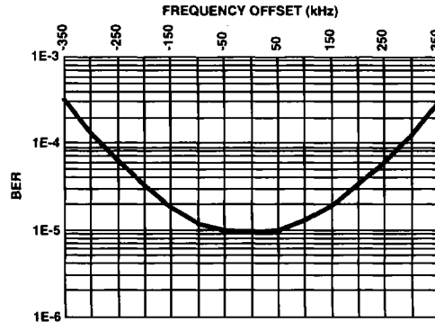
FIGURE 19. BER vs CARRIER OFFSET
