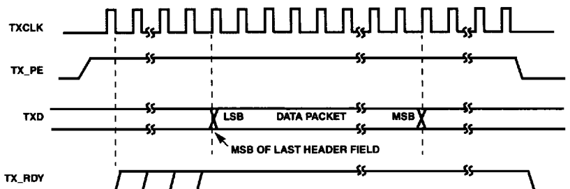
FIGURE 6. TX PORT TIMING (INTERNAL PREAMBLE)
