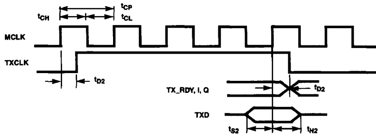
FIGURE 23. TX PORT SIGNAL TIMING
