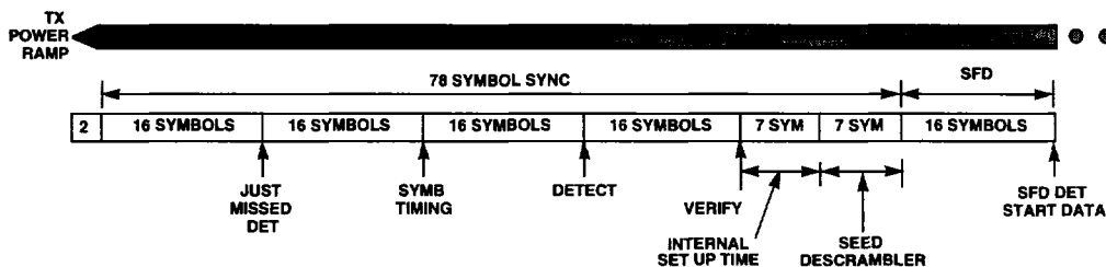
FIGURE 15. SINGLE ANTENNA ACQUISITION TIMELINE
