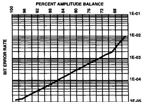
FIGURE 20. I/Q IMBALANCE EFFECTS
