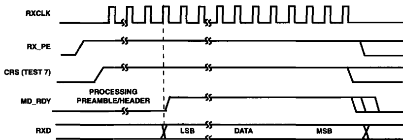
FIGURE 7. RX PORT TIMING
