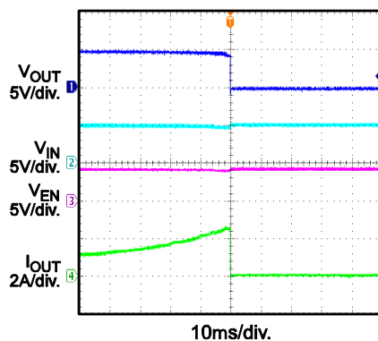
Current Limit Increase I_{OUT} Slowly
