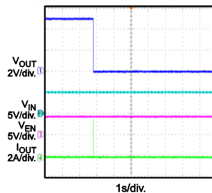
Short Circuit during Normal Operation and Latch off
