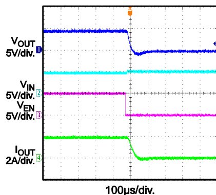
Shutdown through Enable I_{LOAD}=2A
