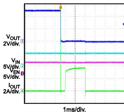
Short Circuit Entry during Normal Operation
