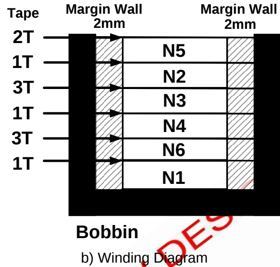
Figure 17: Transformer Structure
