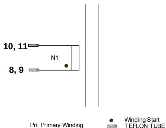
Electrical Diagram
