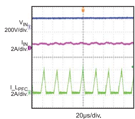
PFC Stage
