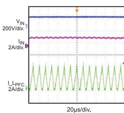
PFC Stage
