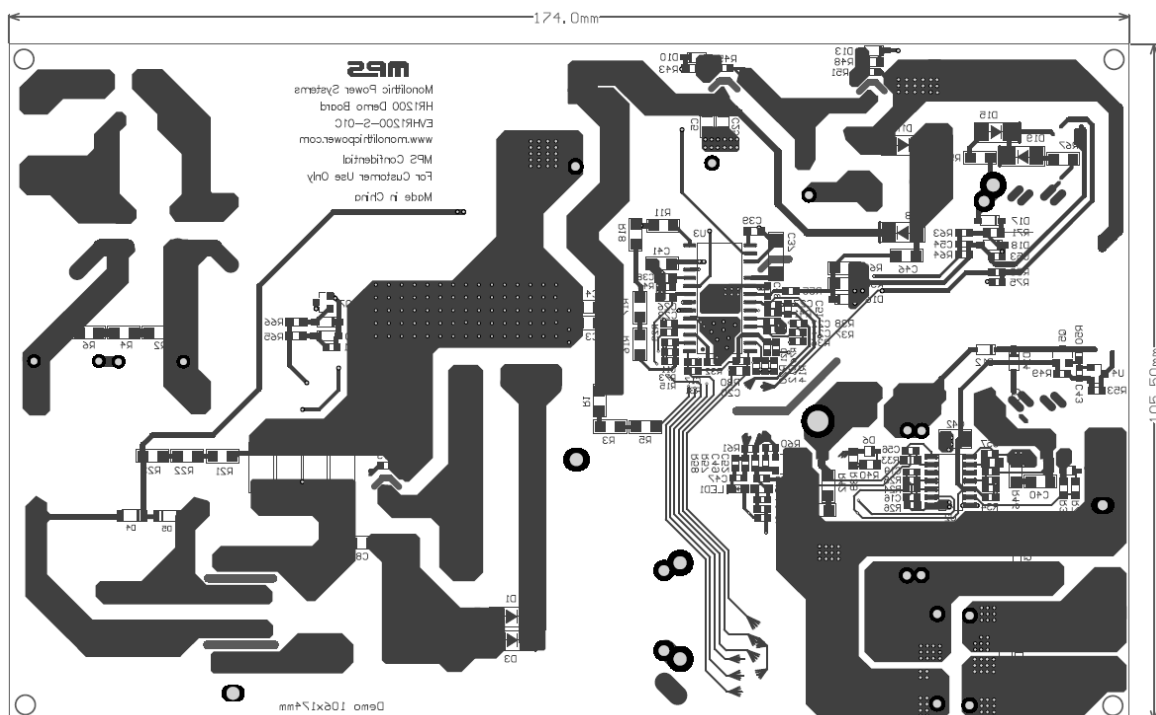
Figure 2: Bottom Layer
