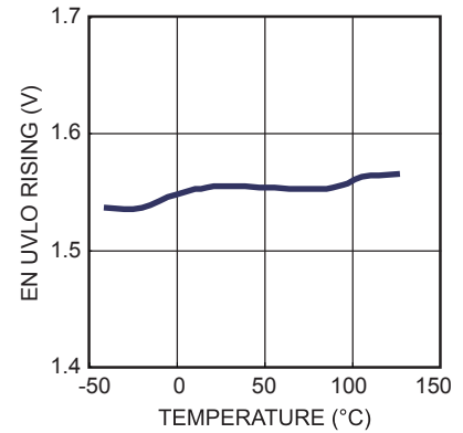
EN UVLO Rising vs. Temperature
