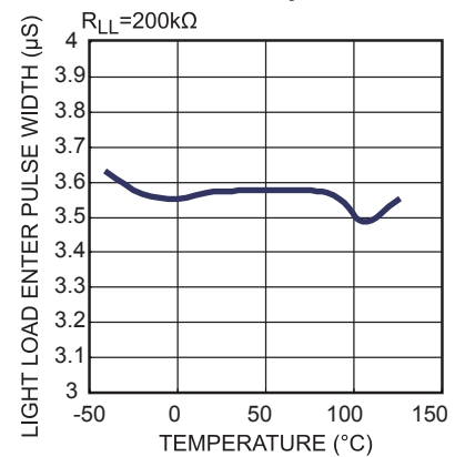
Light Load Enter Pulse Width vs. Temperature
