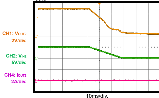
Shutdown through Input Voltage (5V Efuse)
