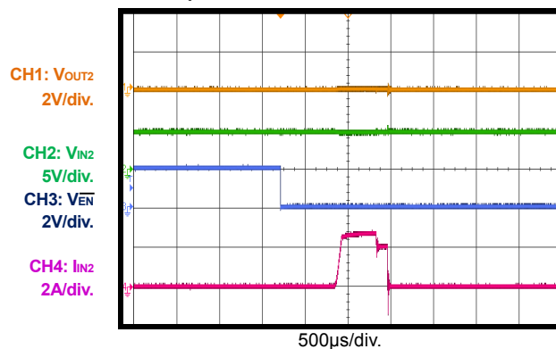
Short Circuit before EN Start-Up (5V Efuse)
