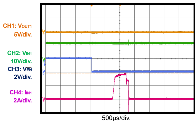
Short Circuit before EN Start-Up (12V Efuse)
