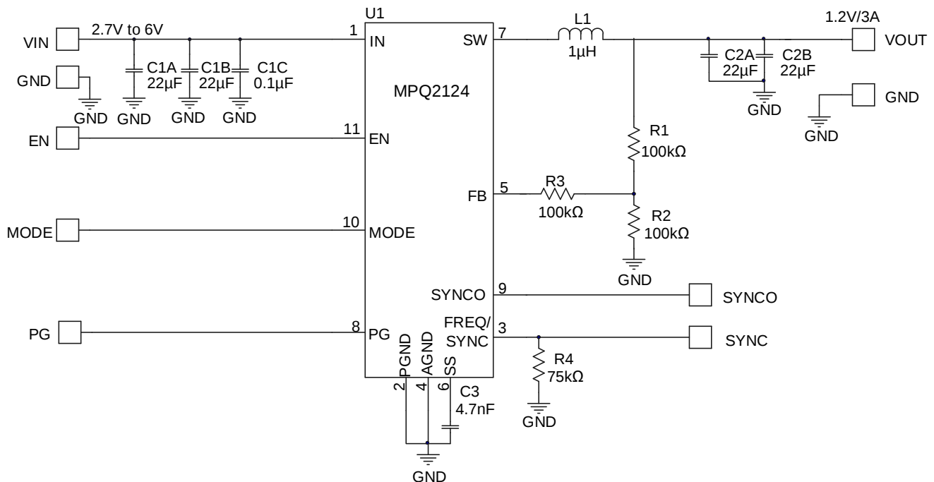
Figure 6: V_{OUT} = 1.2V , I_{OUT} = 3A Application Circuit
