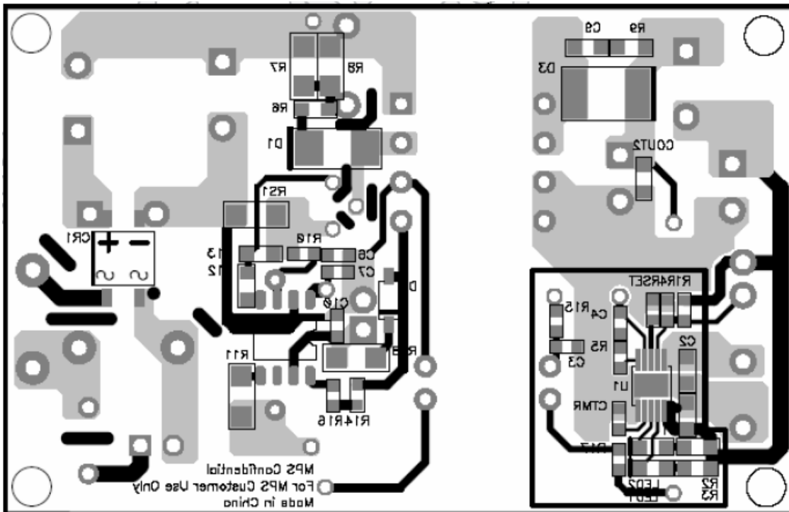
Figure 1—Top Silk
