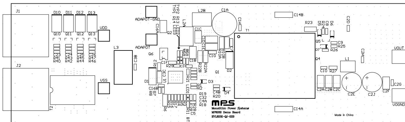
Figure 2: Top Silk
