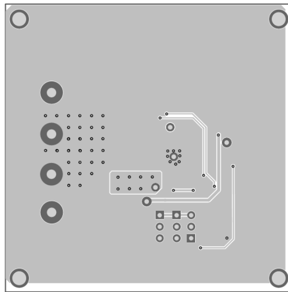
Figure 4: Bottom Layer
