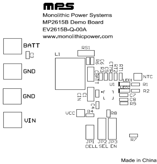
Figure 2: Top Silk
