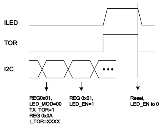
Figure 3: Torch Mode
