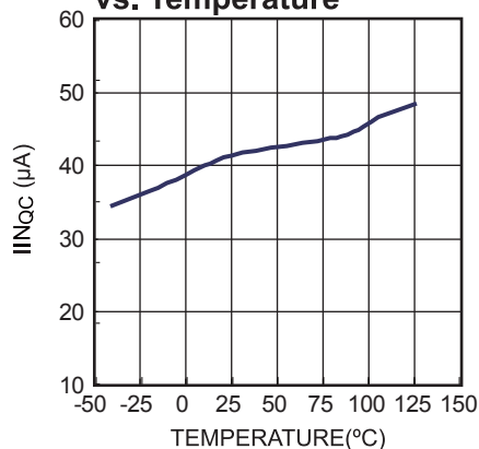
Input Supply Quiescent Current vs. Temperature
