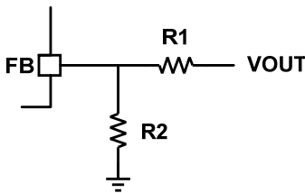
Figure 7: Feedback Network
