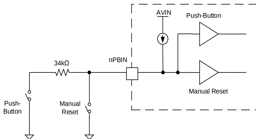
Figure 10: nPBIN Functional Block Diagram
