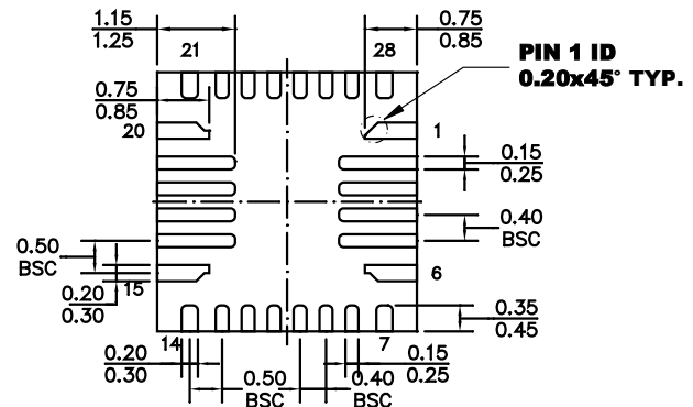
BOTTOM VIEW
