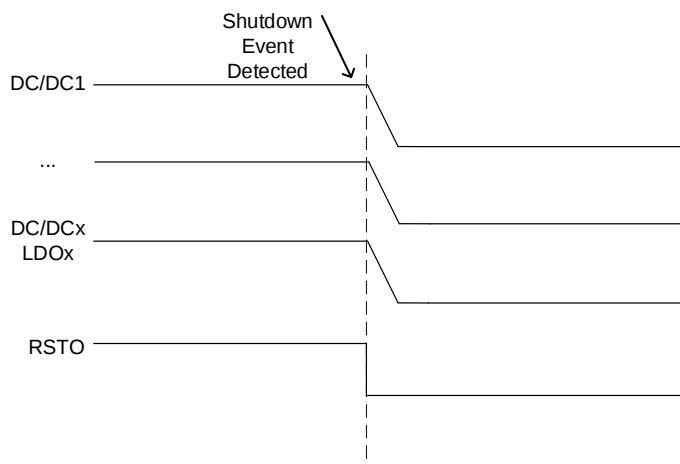
Figure 9: Shutdown Sequence
