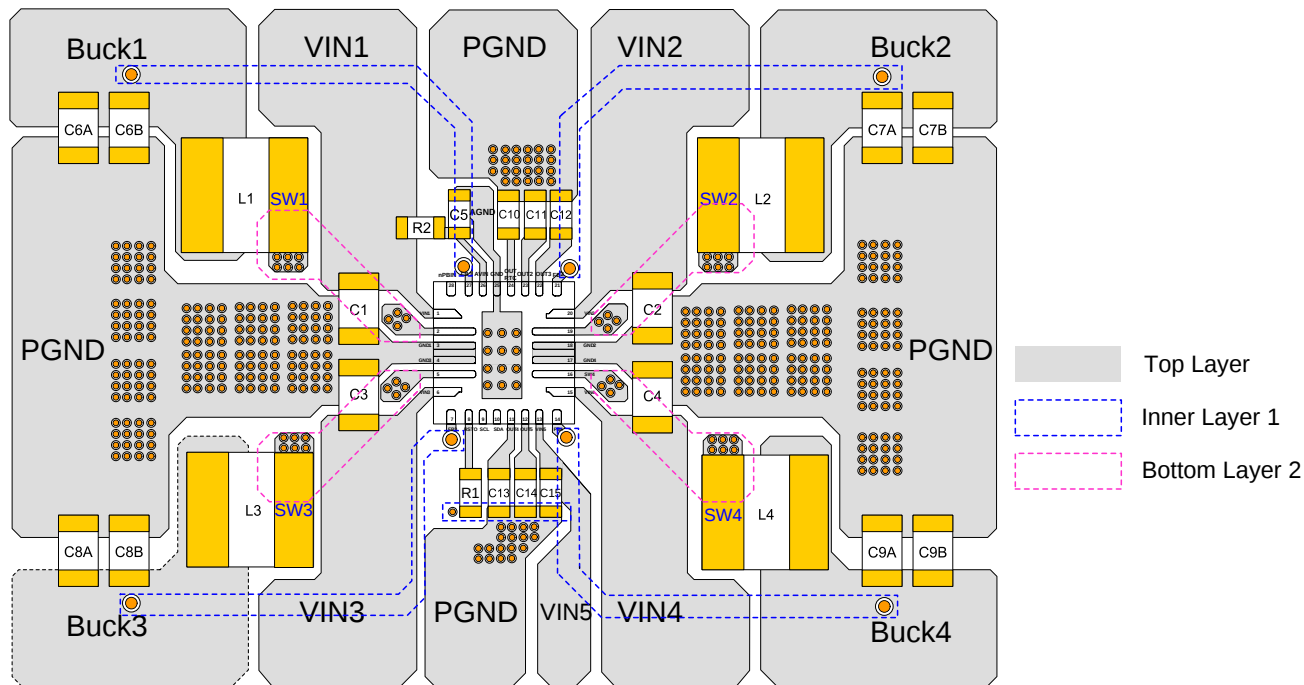
Figure 19: Recommended Layout (14)
