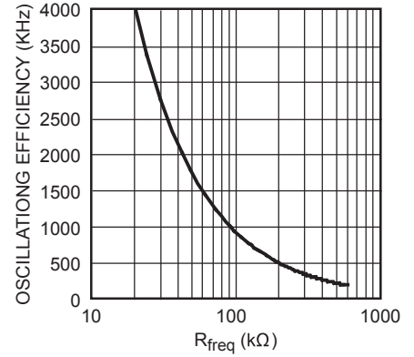
Oscillating Frequency vs R_{freq}
