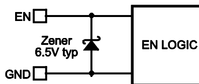
Figure 2: 6.5V Zener Diode Connection
