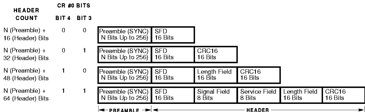
FIGURE 10. PREAMBLE/HEADAR MODES
