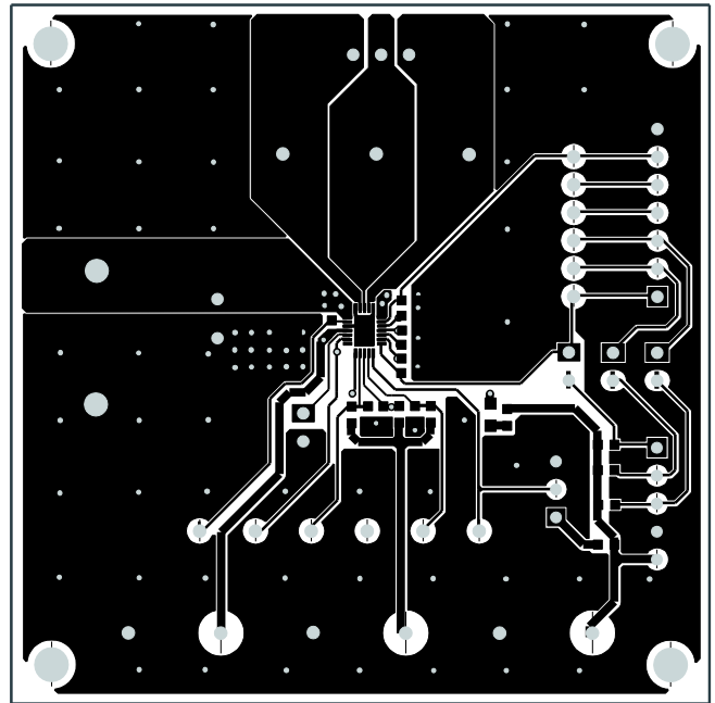
Figure 3: Top Layer
