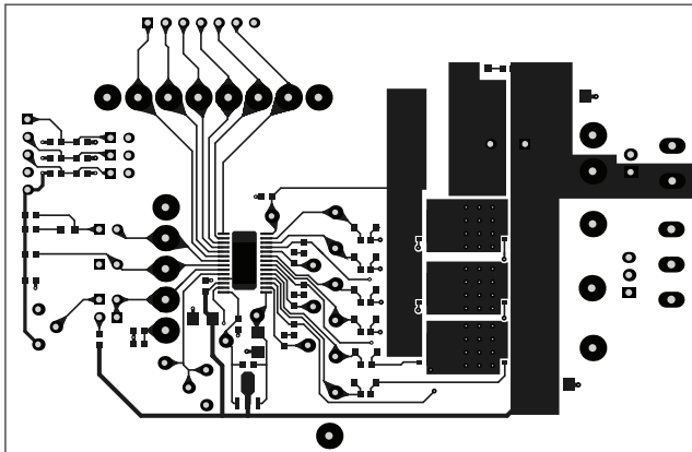
Figure 2: Top Layer
