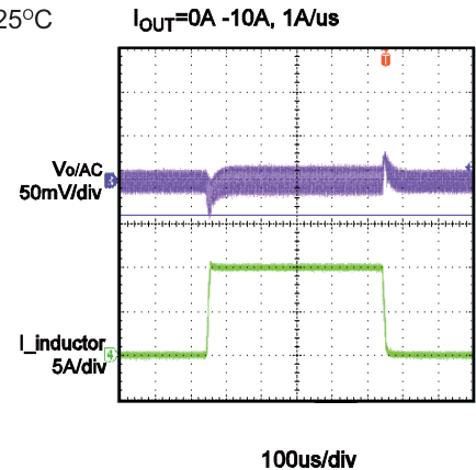
Transient Response
