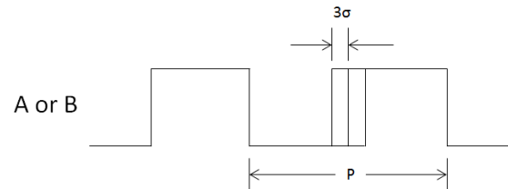
Figure 19: ABZ Jitter
