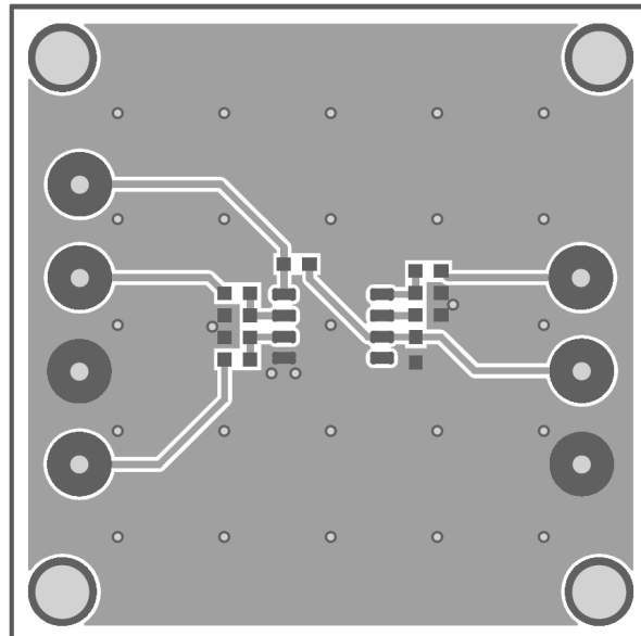
Figure 2: Top Layer
