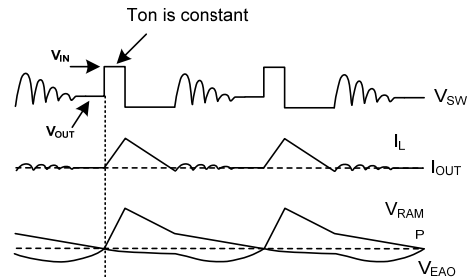
Figure 5: Light-Load Operation
