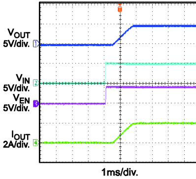
Start-Up through Input Voltage I_{LOAD}=2A
