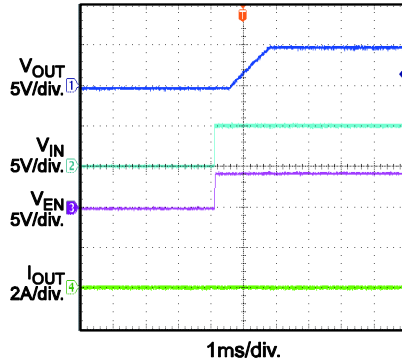
Start-Up through Input Voltage I_{LOAD}=0A
