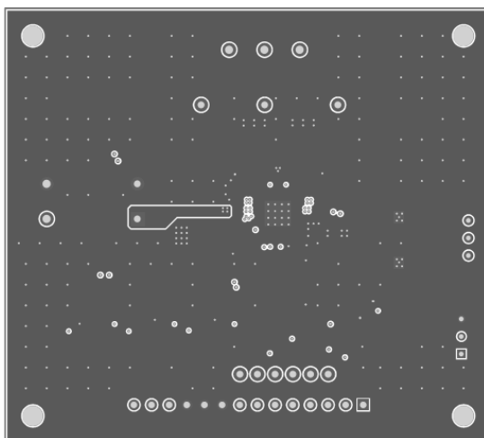
Figure 3—Inner 1 Layer
