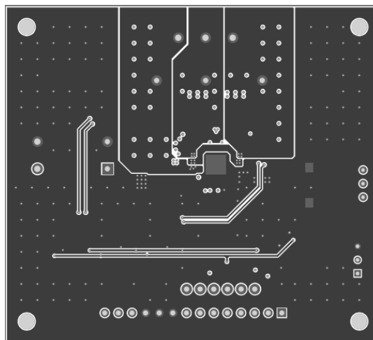
Figure 4—Inner 2 Layer
