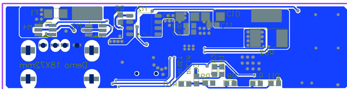
Figure 7: Bottom Layer
