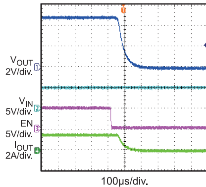
Shutdown Through Enable R_{LOAD} = 3.3\Omega
