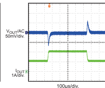
Load Transient Response I_{OUT} = 1A \rightarrow 2A
