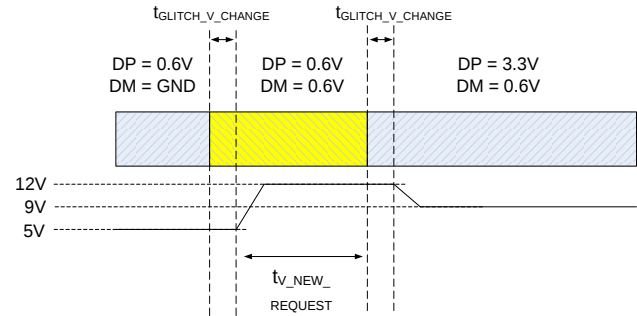
Figure 10: QC Mode Transition
