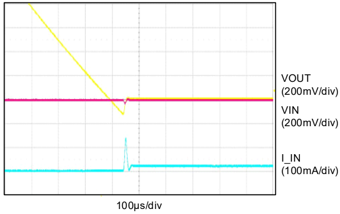
Figure 18. Recovery from True Reverse Current Blocking
