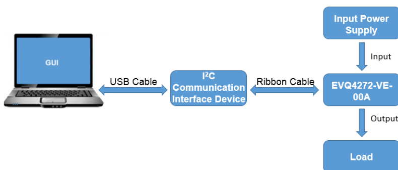
Figure 1: EVKT-MPQ4272 Evaluation Kit Set-Up
