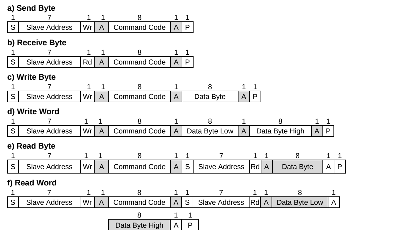
Figure 10: PMBus Message Format
