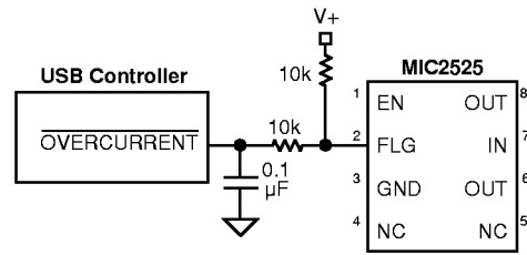
Figure 4. Transient Filter
